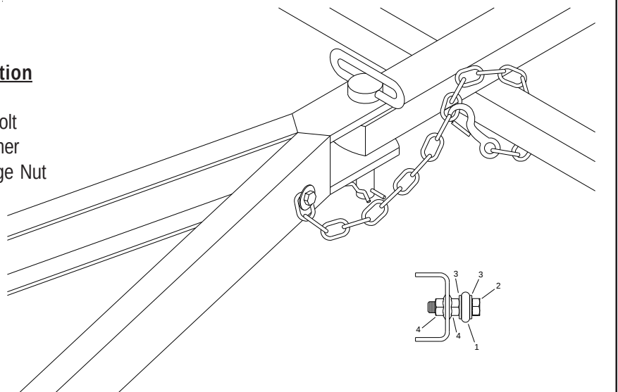
Figure B1 - Attaching the Safety Chain
