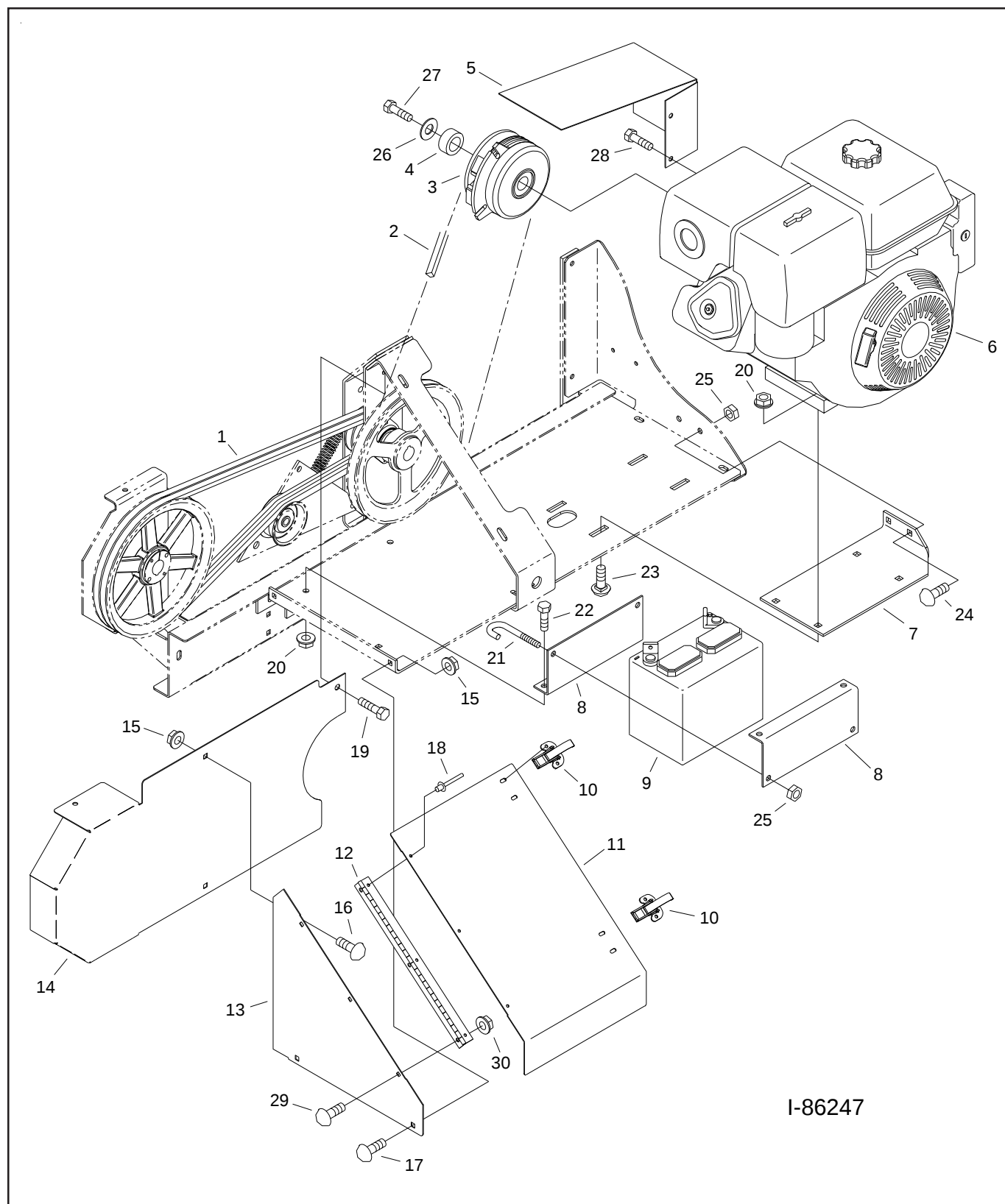
Figure 2 - Engine and Safety Shields
